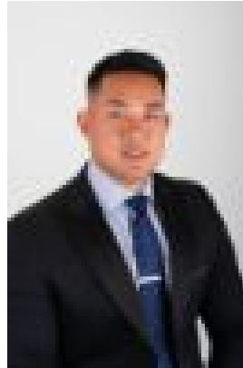
Phi Nguyen 0422778398
